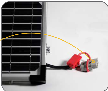
Kits include 12' solar cable with anderson-style connector
